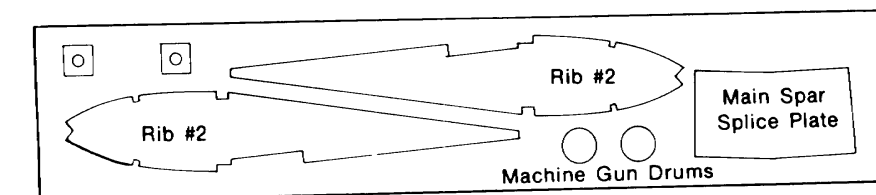
D.C. #11 - 1/16 X 2 15/16 X 18 Ply
